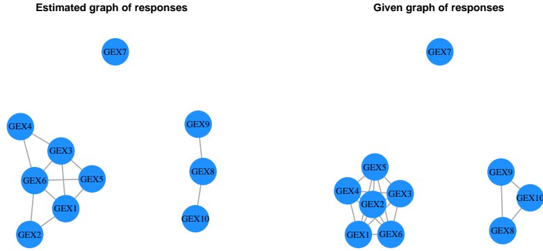
Figure 5: The estimated structure of the ten response variables is visualized by plot(fit, estimator = "Gy", type = "graph") with \hat{\mathcal{G}} thresholded at 0.5 (left). The true structure is shown with plotGraph(Gy) , where Gy is the true adjacency matrix (right).
